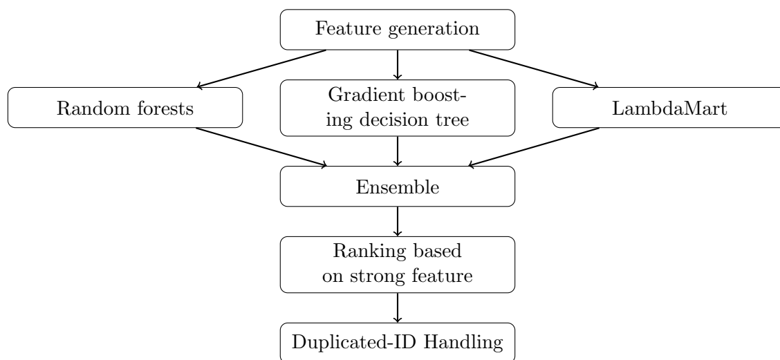
Figure 2: The detailed architecture of our approach.
